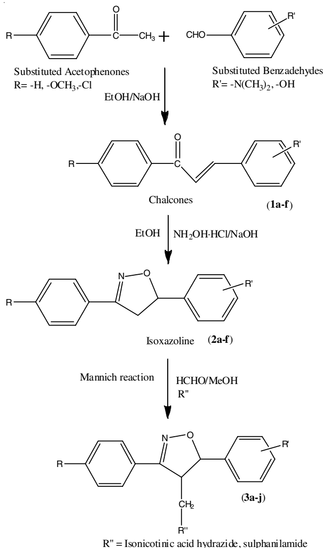
Scheme-I: Synthesis of substituted isoxazole derivatives
