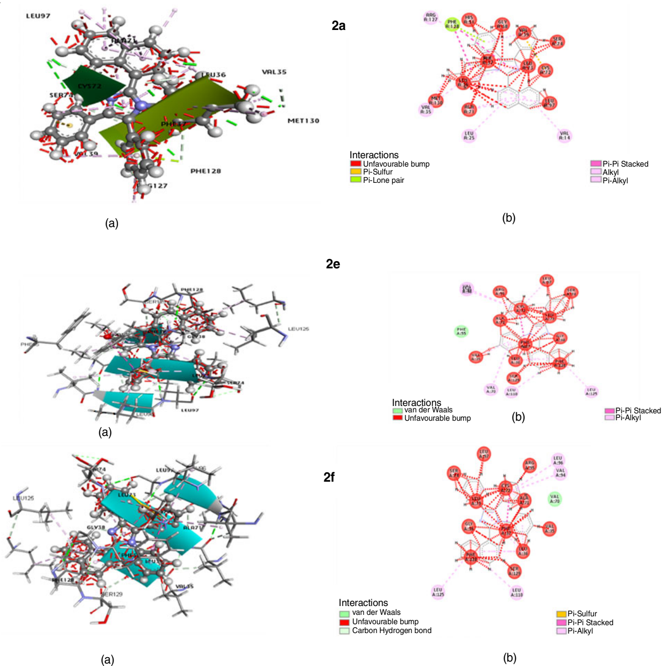
Fig. 1. (a) Three dimension and (b) Two dimension binding interaction of the compounds 2a , 2e , 2f with ligands of receptor 3MNG
