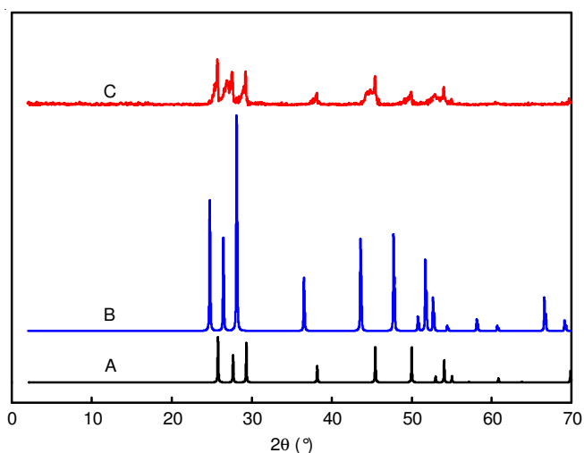
Fig. 2. XRD patterns of (A) \gamma\text{MnS} (B) CdS and (C) \text{Mn}_{1-x}\text{Cd}_x\text{S} ( x = 0.18 )
