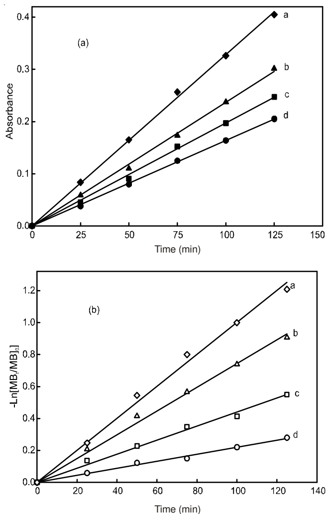
Fig. 4. Linear form of first order decolorization at 664 nm of methylene blue (200 mL, 15 \mu M) in presence of (a) visible light irradiation and in presence of (b) UV light irradiation. The lines a, b, c and d indicate the presence of 0.2 g Mn_{1-x}Cd_xS ( x = 0.18 ), TiO_2 , ZnO and CdS photocatalysts, respectively
