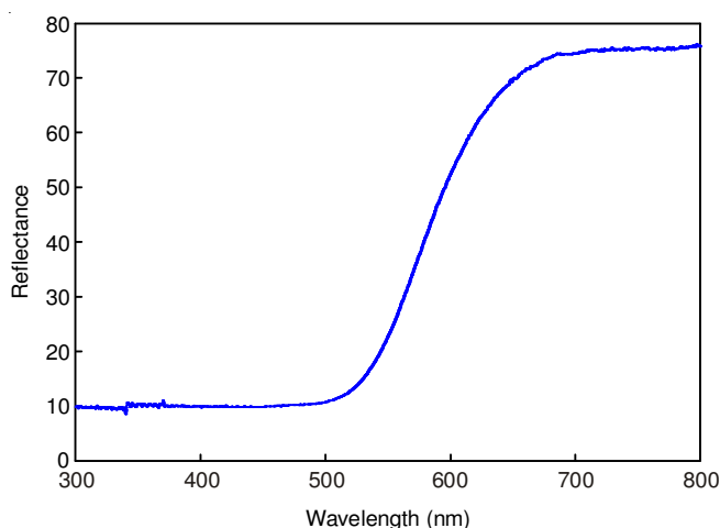
Fig. 6. Reflectance spectra of the as prepared Mn_{1-x}Cd_xS ( x = 0.18 )
