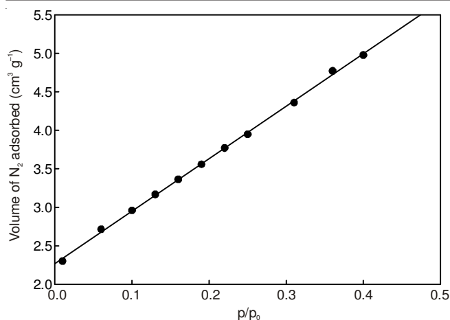
Fig. 5. BET isotherm of as prepared Mn_{1-x}Cd_xS ( x = 0.18 ) catalyst
