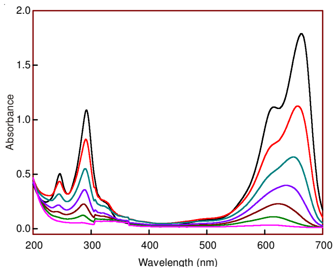
Fig. 3. The temporal absorption spectrum changes of methylene blue taking place under visible light irradiation. The lines indicate the change of decolorization/degradation every 25 min intervals. Initial concentration of methylene blue: 15 \mu M (200 mL), Mn_{1-x}Cd_xS ( x = 0.18 ); 0.2 g, pH: 7.5
