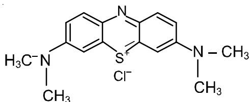
Fig. 1. Molecular structure of methylene blue
