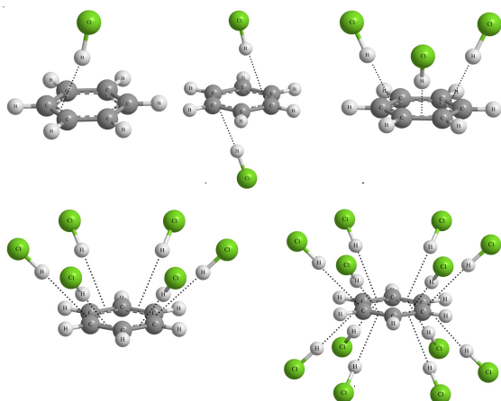
Fig. 1. Structure of model C_6H_6 \cdots n HCl ( n = 1, 2, 3, 6, 12 )
