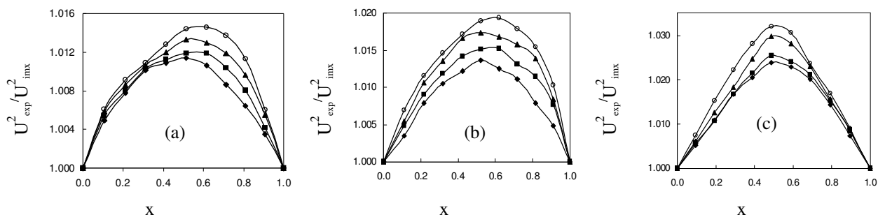
Fig. 1. Variation of U_{\text{exp}}^2/U_{\text{inx}}^2 , against mole fraction of N-methyl-2-pyrrolidone(x) for the system N-methyl-2-pyrrolidone + chlorobenzene (a), N-methyl-2-pyrrolidone + bromobenzene (b) N-methyl-2-pyrrolidone + aniline (c) at temperatures 303.15 K, \blacklozenge , 308.15 K, \blacksquare , 313.15 K, \blacktriangle , 318.15 K \circ
