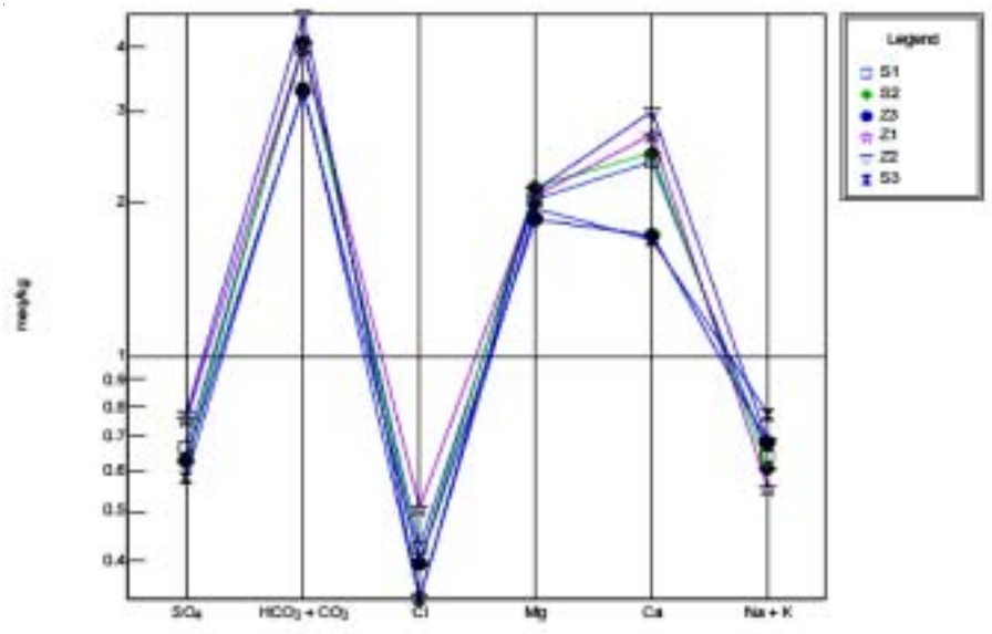
Fig. 2. Scholler diagram
