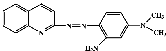
Fig. 1. Structure of 2-(2-quinolyldiazo)-5-dimethylaminoaniline
